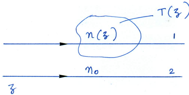
INTERFEROMETRY {OPTICAL PATH DIFFERENCE}
